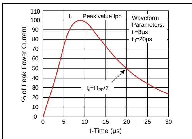
Figure 1. Pulse Waveforms
